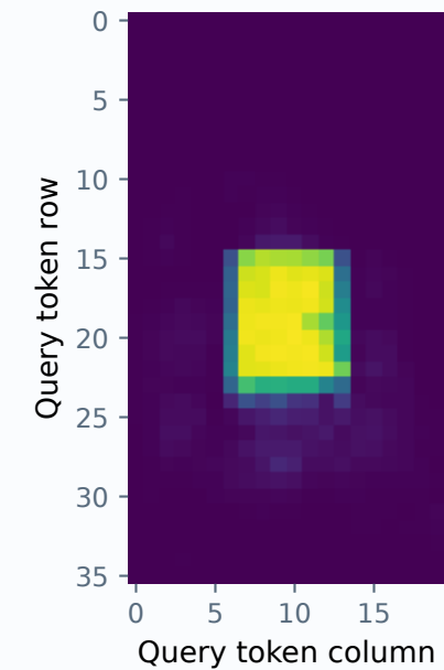
Paired with the correct reference
